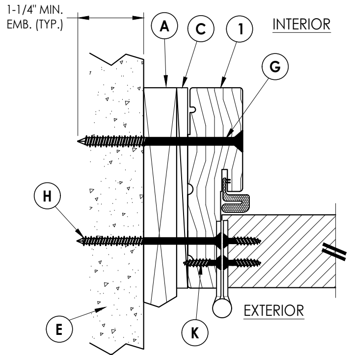
2 HORIZONTAL CROSS SECTION 2 Outswing shown - Inswing similar 1X Buck Construction
